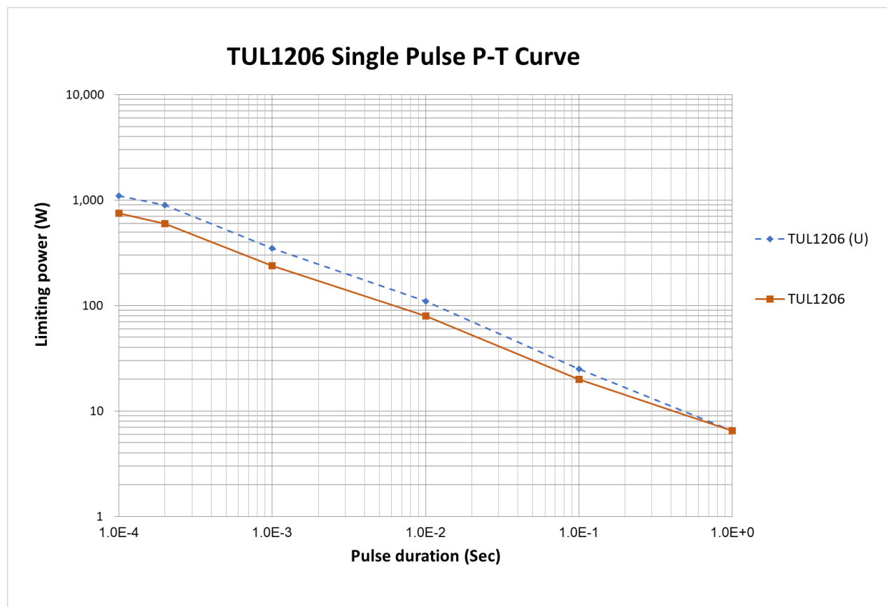
TUL1206 P-T curve; Pulse Limiting power vs duration
