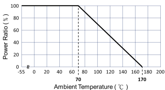
Derating Curve
