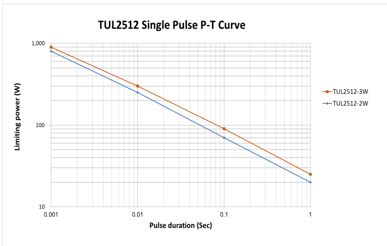
TUL2512 P-T curve; Pulse Limiting power vs duration
