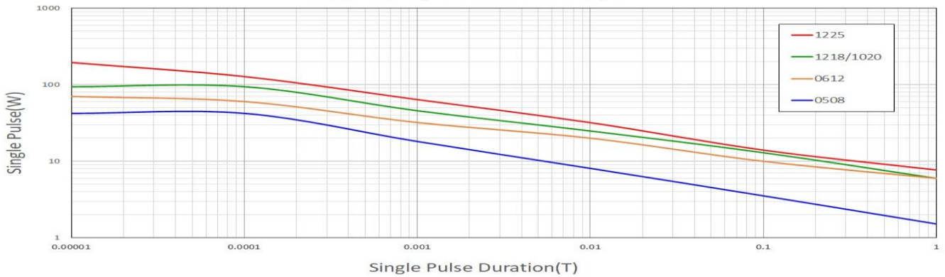
CRW-Z Single Pulse P-T Graph
